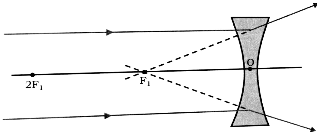
Object at infinity
